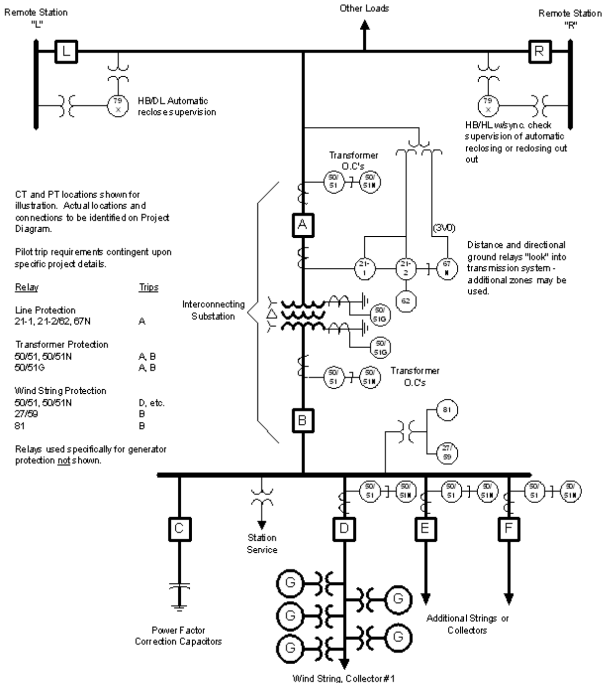
Figure 13.--- Integration of a Typical Wind Generation Facility to a 69 kV or 115 kV Transmission Line Through a YG-Δ-YG Transformer
