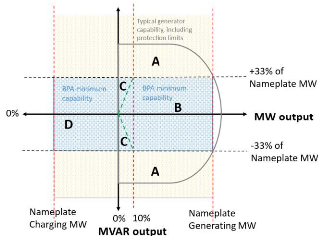
Figure 1.--- Required Reactive Power Capability at POI (when the POI is inside a defined voltage band around the scheduled voltage))
