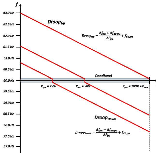
Figure 8.--- Frequency Response from NERC IBR Guidelines
