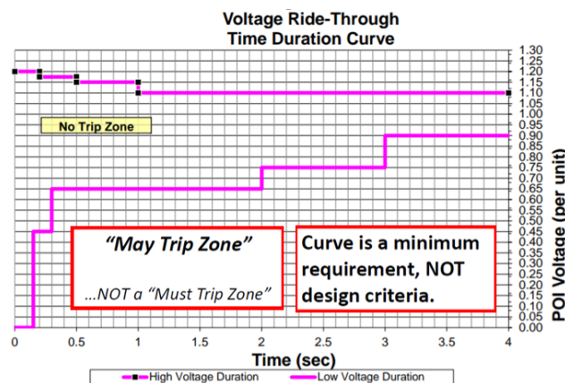
Figure 7.--- LVRT Duration curve, Modified from NERC PRC-024
