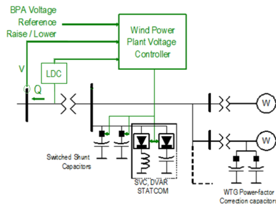
Figure 5.--- Type 1/2 Wind Turbine Reactive Power Control with FACTS-device Controllable Plant-level Reactive Compensation (SVC, STATCOM, DVAR, etc.)
