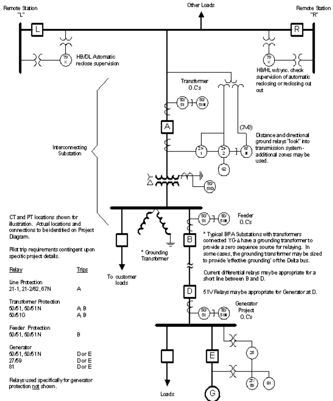
Figure 10.--- Integration of Generation into a Low Voltage Substation Protected by a High Side Circuit Breaker and Connected to a Transmission Line Through a YG-Δ (as shown) or YG-Δ-YG Transformer
