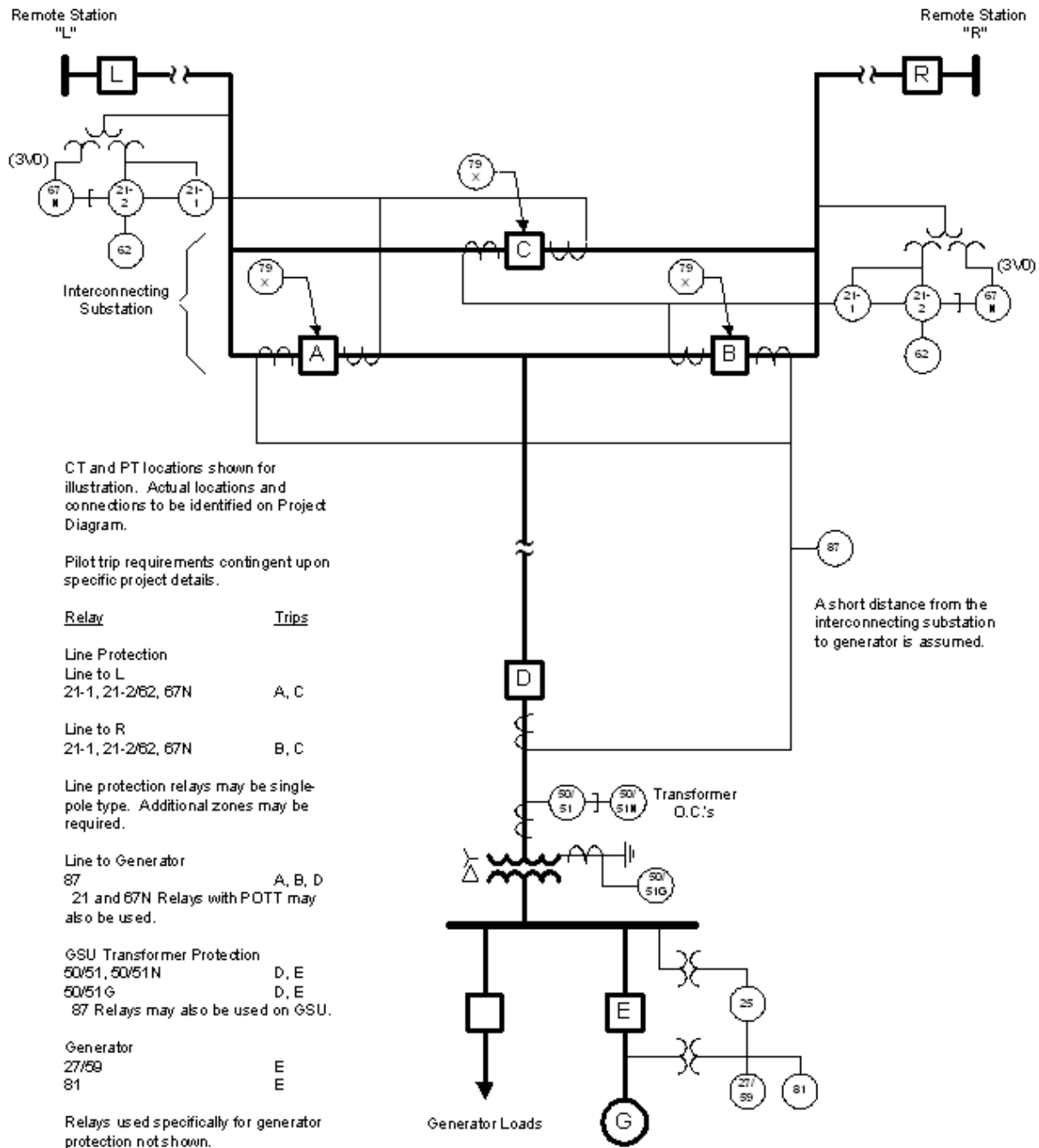
Figure 9.--- Integration of Generation into a Transmission Level Substation
