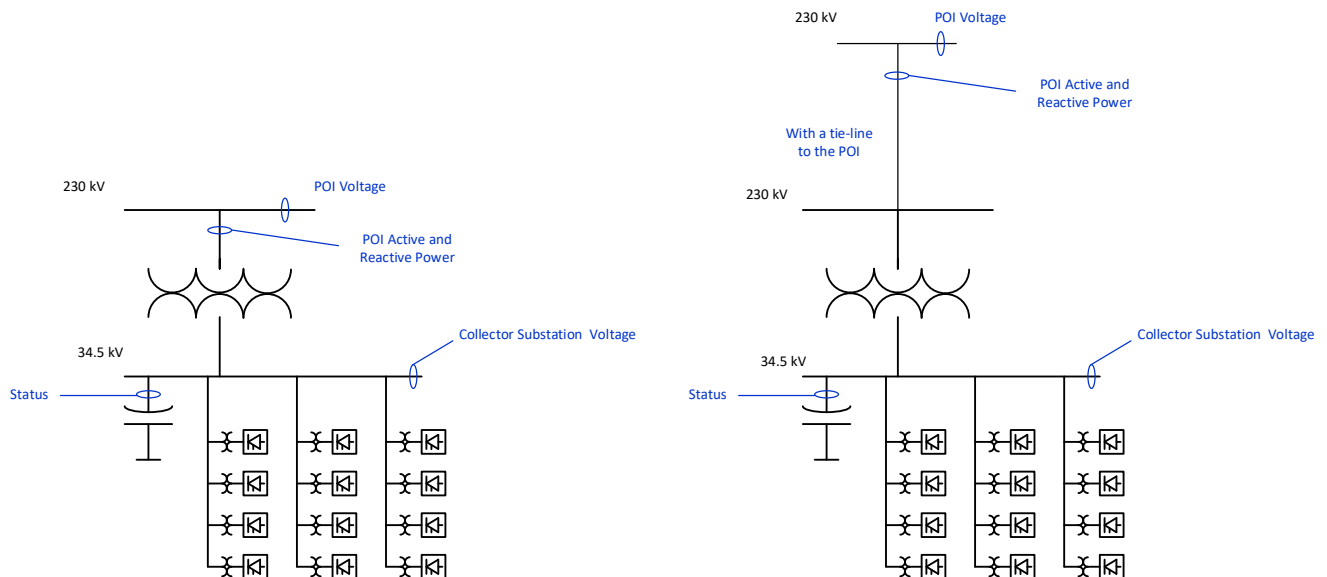
Figure 3.--- Example of Important Reference Quantities Required for Acceptable POI Voltage Control
