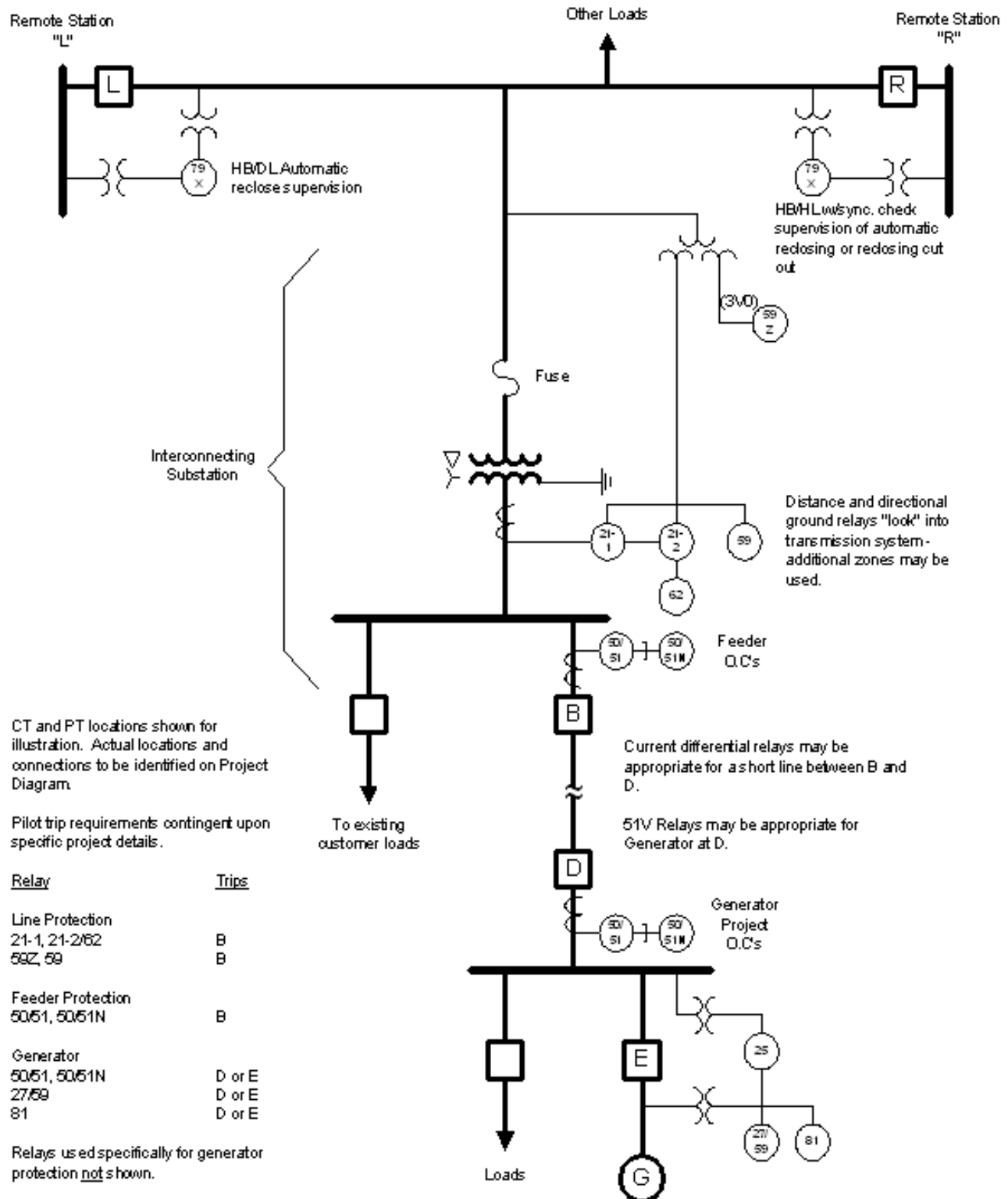
Figure 11.--- Integration of Generation to an Existing Low Voltage Substation Connected to the Transmission line Through a Fused Δ-YG Transformer
