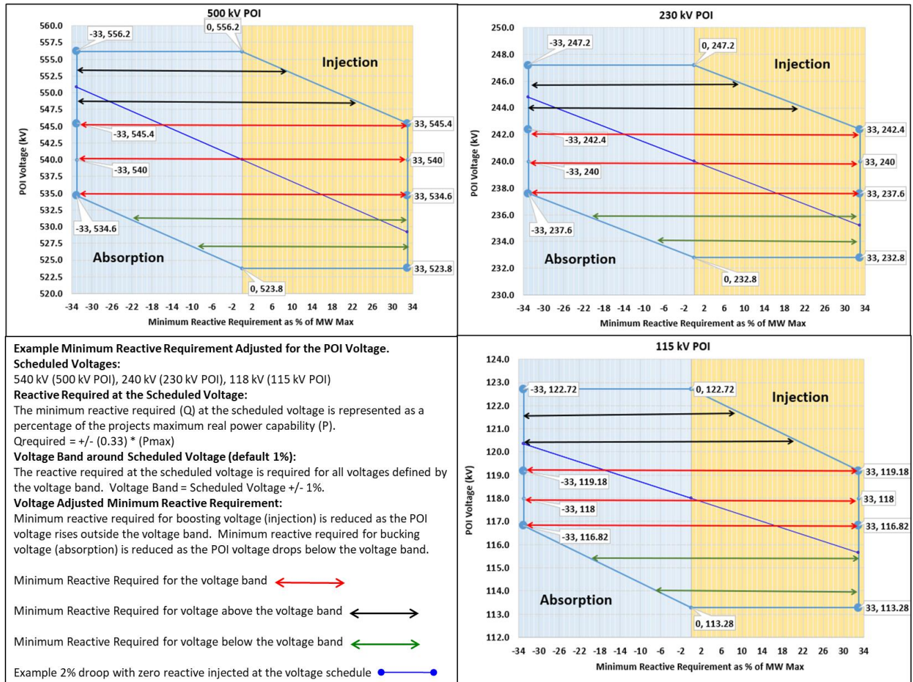
Figure 2.--- Minimum Reactive Required at the POI Adjusted for POI Voltage (Examples for a 500 kV POI, 230 kV POI, and 115 kV POI). Note that requirements for technologies unable to meet the reactive capability requirements at low power outputs such as type 3 wind turbines are not represented in these plots.
