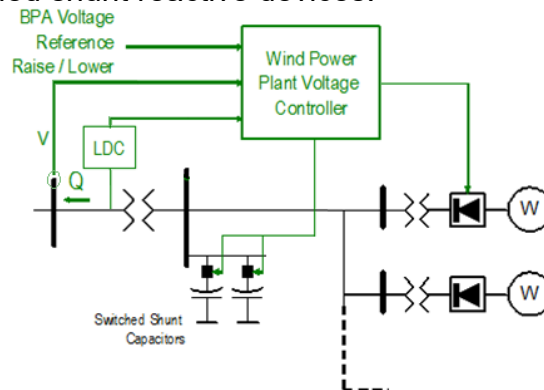
Figure 4.--- Type 3/4 Wind Turbines Providing Primary Generator Reactive Power
