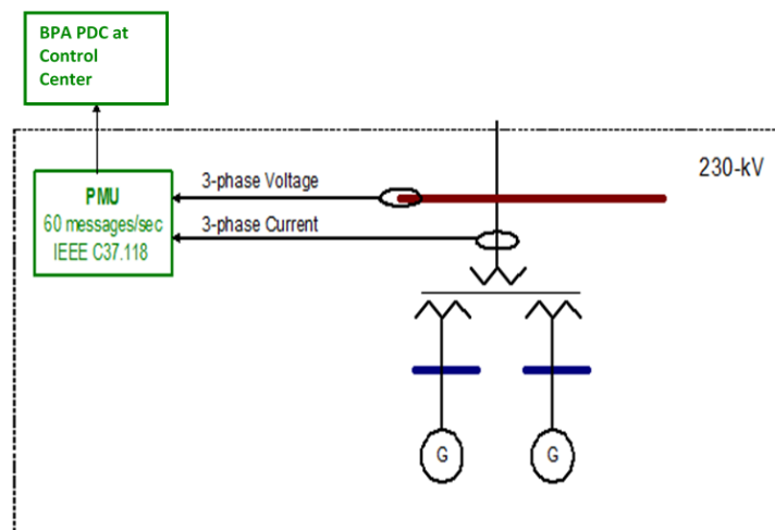
Figure 14.--- Example Phasor Measurement Unit (PMU) Installation
