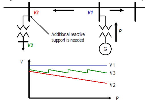
Figure 6.--- Voltage Impact on Line Connected Load for VER Generation
